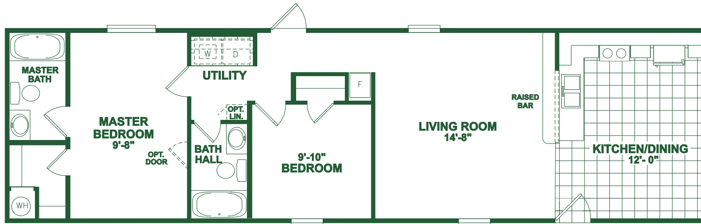
MODEL: 318 16'x56' (60' OVERALL) APPROX. 868 SQ. FT. 2 BEDROOMS, 2 BATHS
