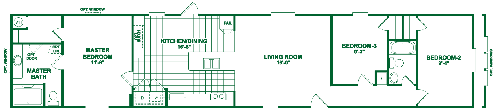
MODEL 320 16'x76' (80' OVERALL) APPROX 1178 SQ. FT. 3 BEDROOMS, 2 BATHS
